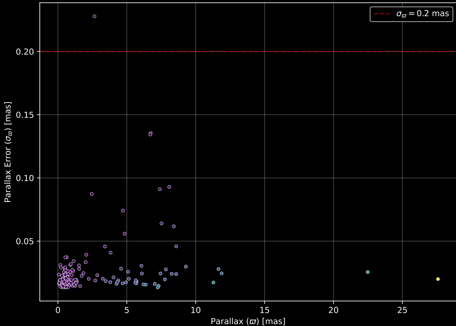
APOGEE DR17 Field: [208+20_MGA] Parallax Quality (n= 163)
