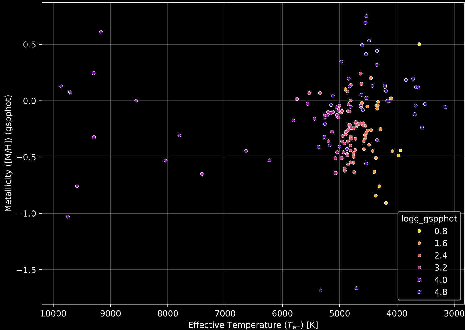
APOGEE DR17 Field: [208+20_MGA] Stellar Population Parameters (n= 163)
