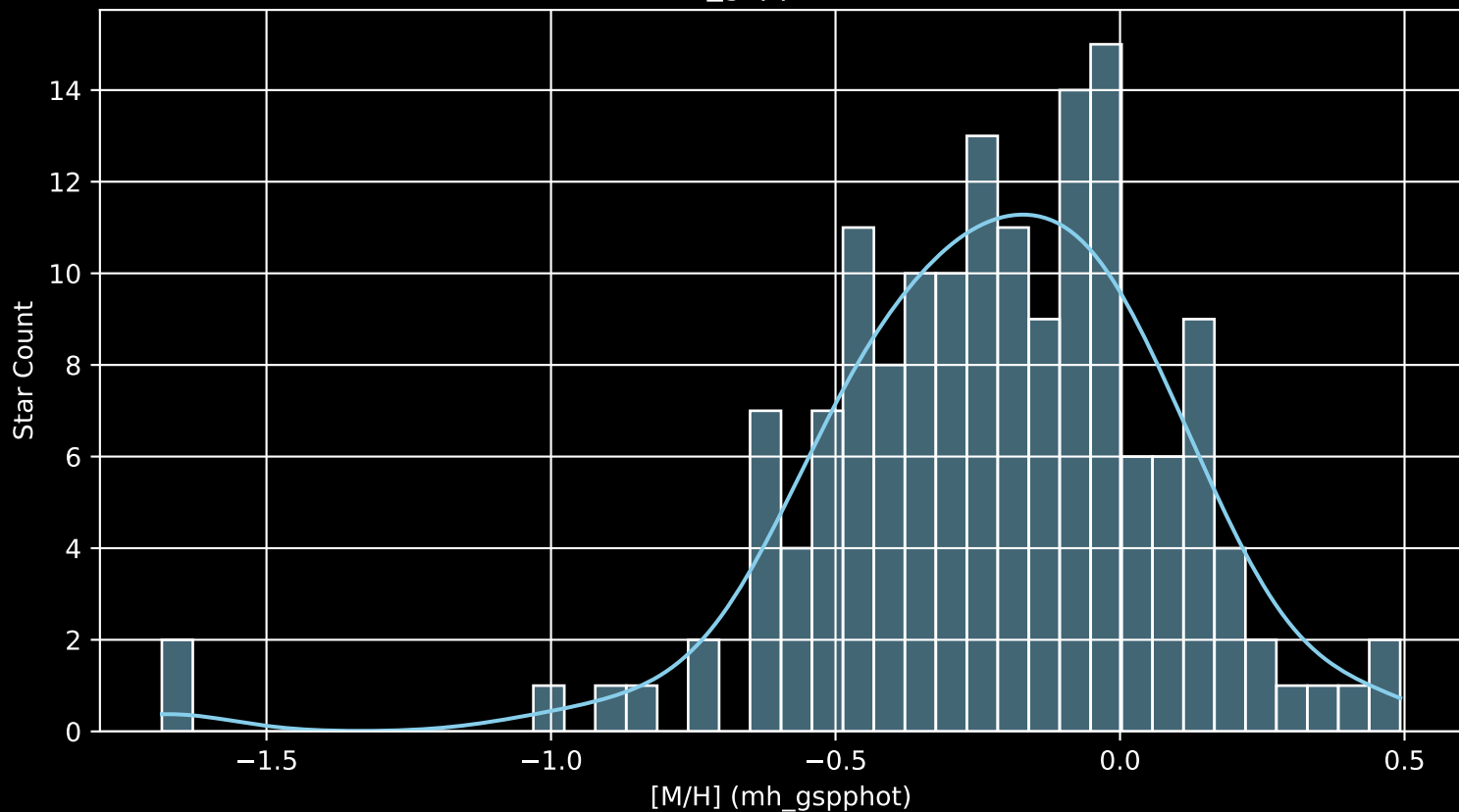
APOGEE DR17 Field: [208+20_MGA [M/H] (mh_gspphot) (n= 158)
