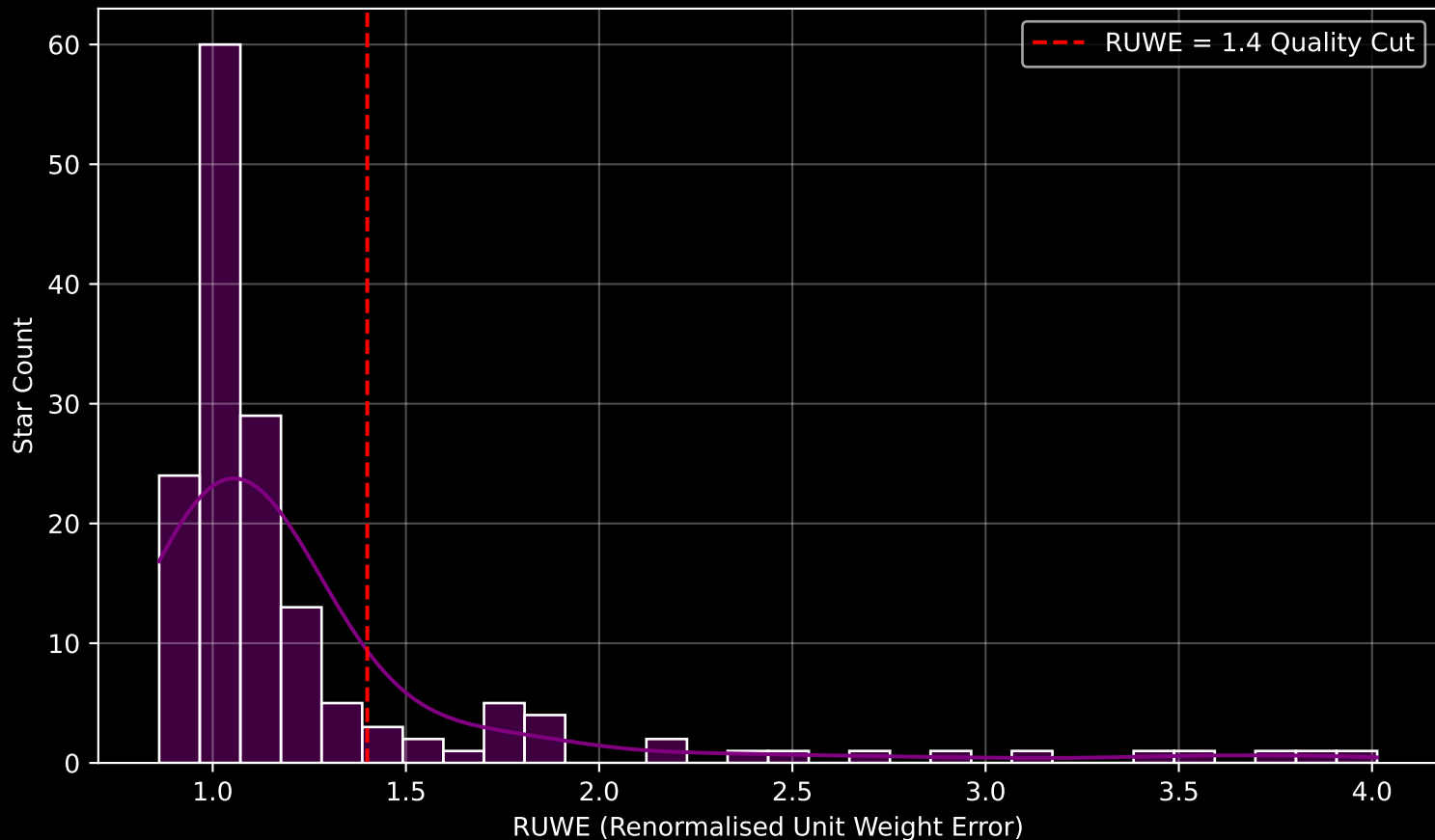
GAPOGEE DR17 Field [208+20_MGA] RUWE Distribution (n= 158)
