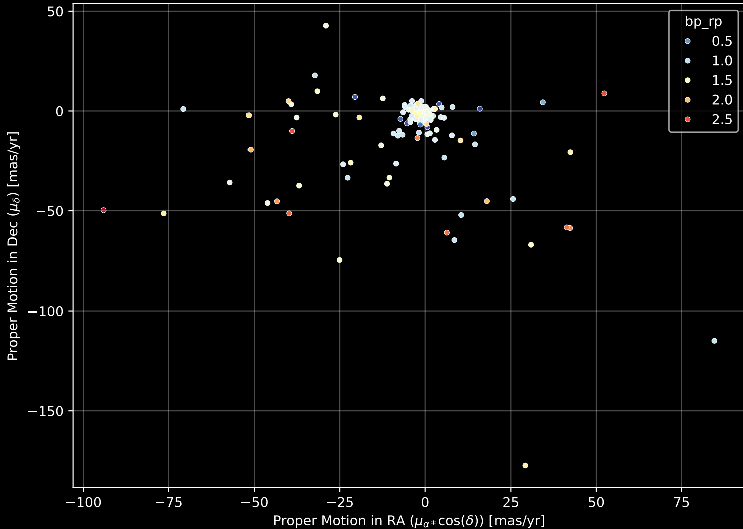
APOGEE DR17 Field: [208+20_MGA] Proper Motion Diagram (n= 163)
