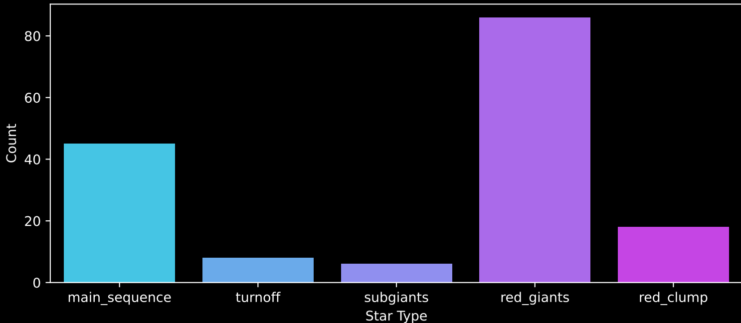
APOGEE DR17 Field: [208+20_MGA] Count plot of Star Type
